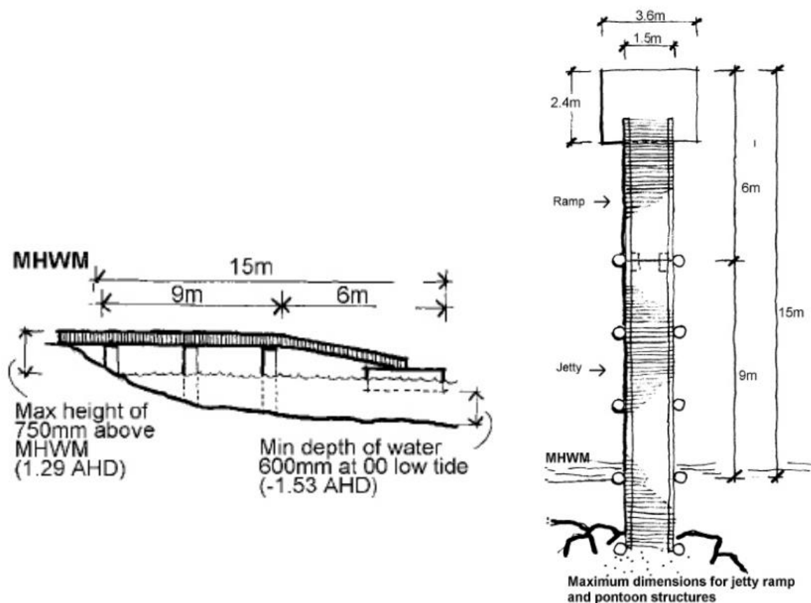
Figure 11: Jetty, ramp and pontoon structures maximum dimensions
